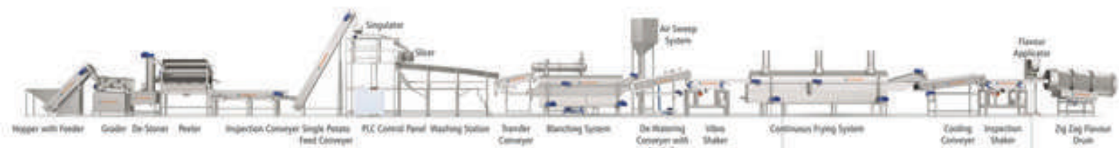
Potato Chips Line
